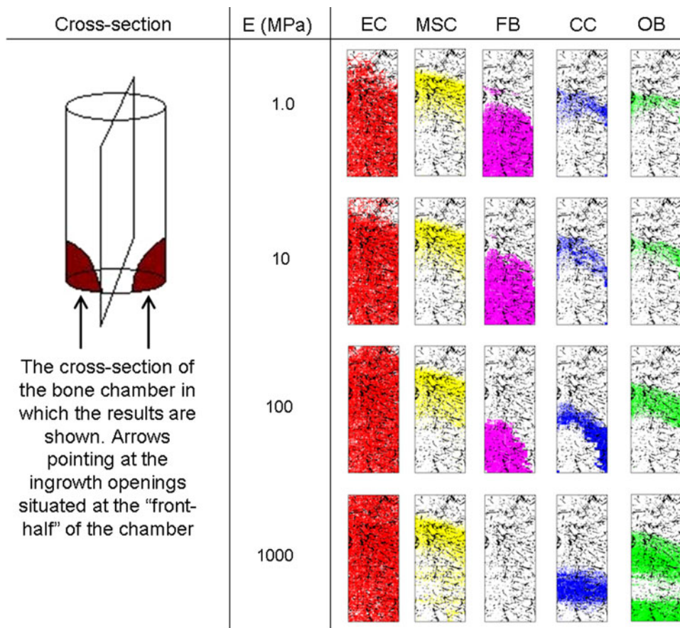
Fig. 2 Mid-cross-sections of the chamber where the coloured lattice points illustrate endothelial cells (EC), mesenchymal stem cells (MSC), fibroblasts (FB), chondrocytes (CC) and osteoblasts (OB). The black lattice points scattered in the entire chamber denote the scaffold occupying the chamber
