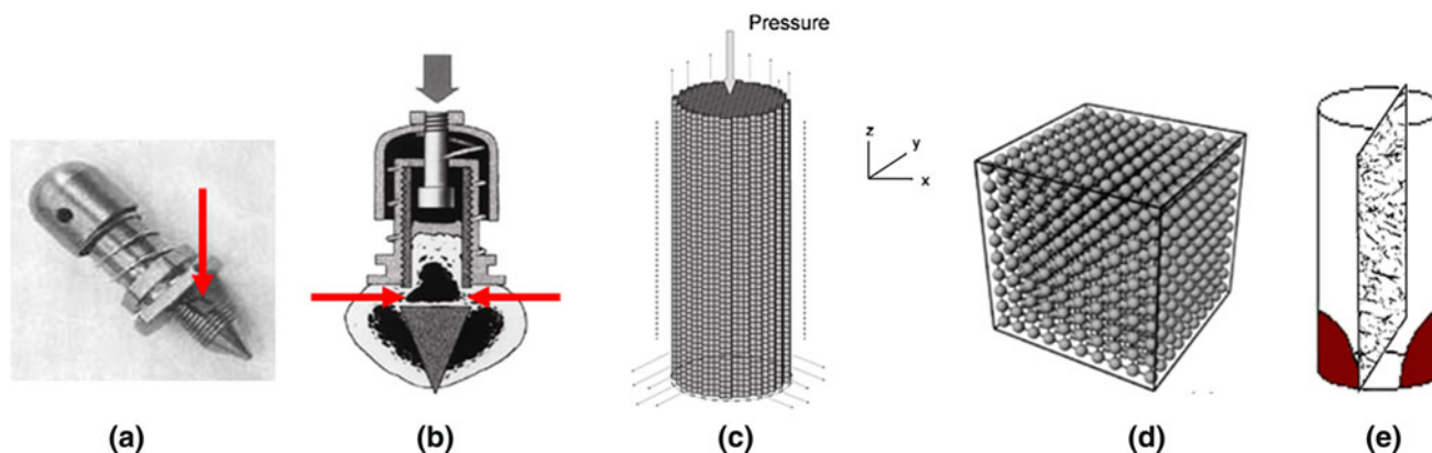
Fig. 1 a The bone chamber, where the arrow points at an ingrowth opening. b Cross-section of the bone chamber [15] where the thin arrows point at the ingrowth openings and the thick arrow points at the piston by which loading is applied. c FE-model of the interior of the bone chamber where the chamber wall was modelled as boundary conditions; ↑↑↑↑: free fluid flow; ↑↑↑↑: u_x = u_y = 0 ; ----:
